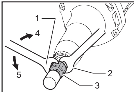
► 1. Wrench 19 2. Wrench 13 3. Collet nut 4. Tighten 5. Loosen
